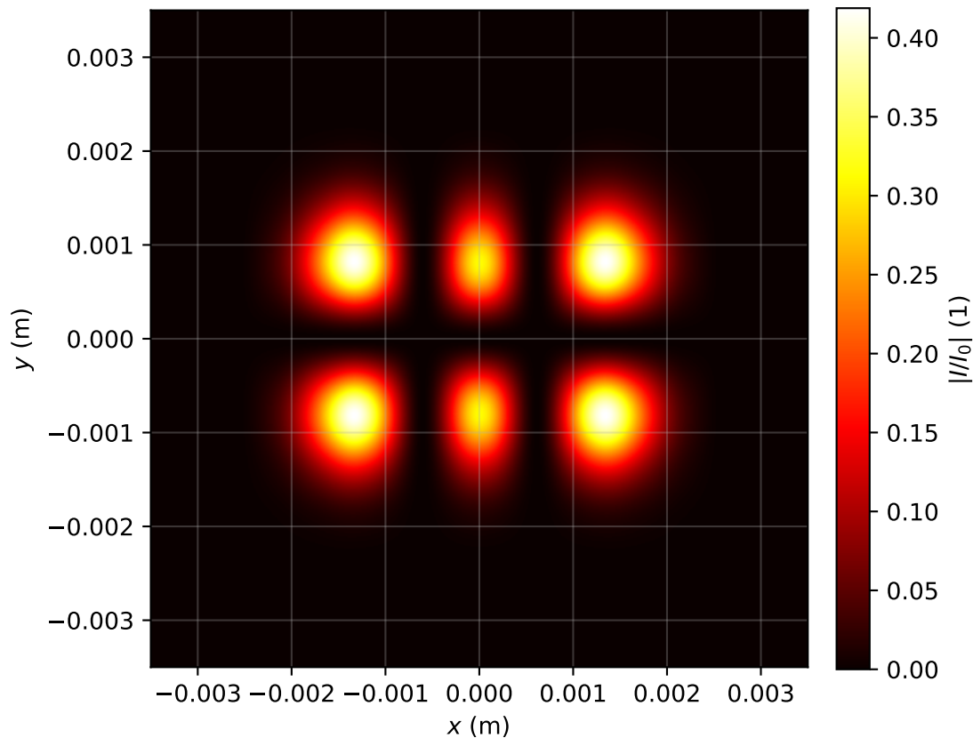
Intensity profile I(x, y, z = 2.707)/I_0 , P_{in}=1.0P_{cr} , artificial time
